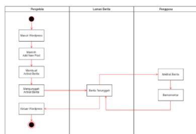
Gambar 6. Activity Diagram Laman Berita
